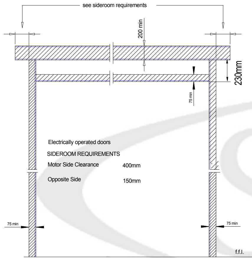
Elevation from inside building
