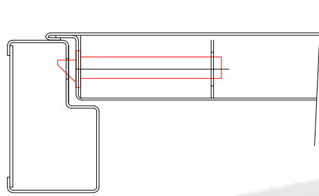
OPENING SIDE DETAIL
