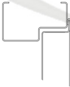
TOP DETAIL HEADSECTION
