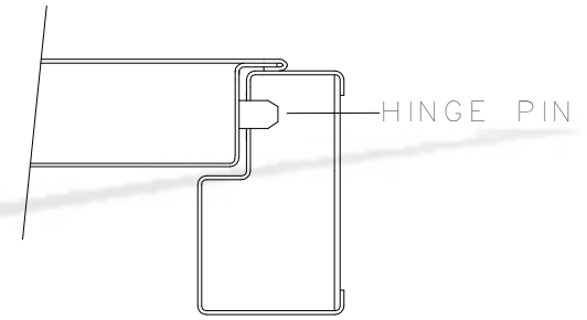
HINGE SIDE DETAIL
